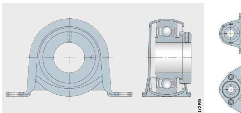
Figure 1 Plummer block housing unit, sheet steel housing
