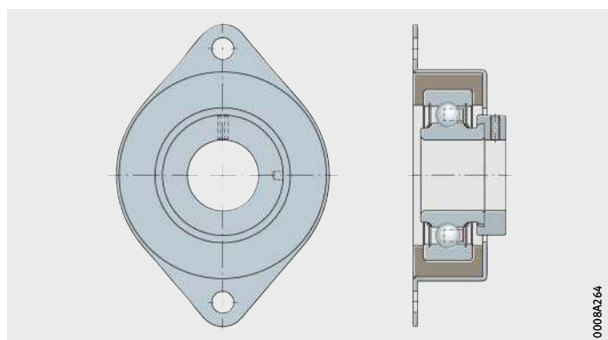
Figure 3 Flanged housing unit with rubber interliner
