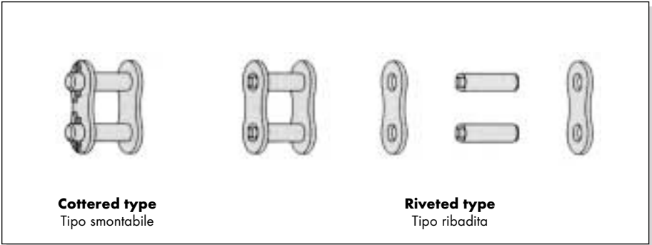
Pict. 3 Pin link. Fig. 3 Maglia esterna.
