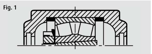
Fig.1: In the fixed plummer block, to prevent axial displacement of the bearing, 2 locating rings are installed, one on either side of the bearing. Locating rings are manufactured in aluminium.
